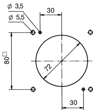
Hole pattern
